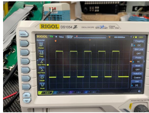
9600 baud
