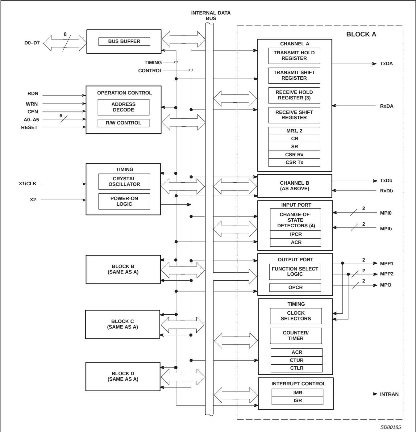
Figure 2. Block Diagram
